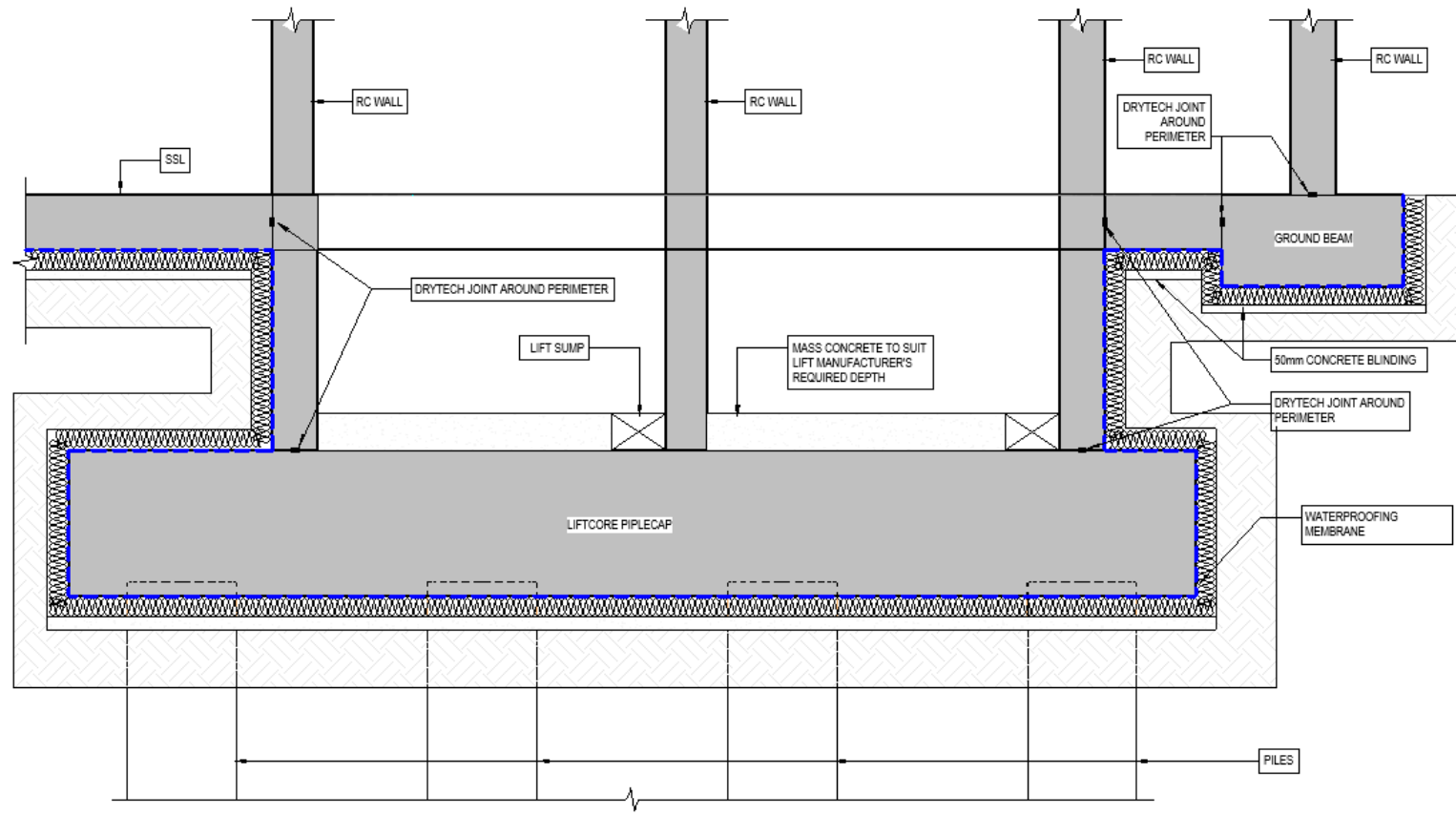
Typical Lift Pit (In-Situ RC Frame Superstructure)
