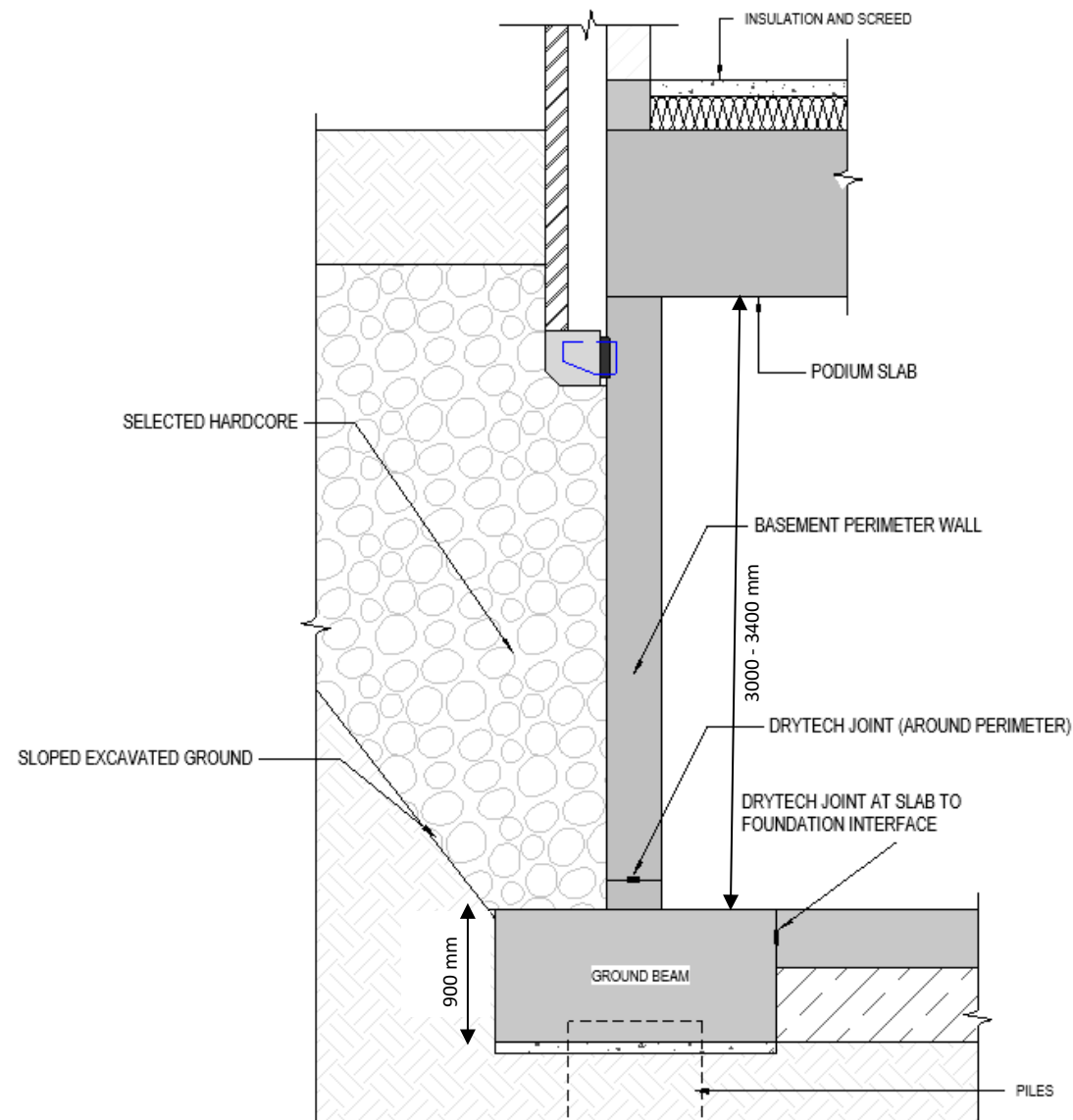
Typical Basement Wall
